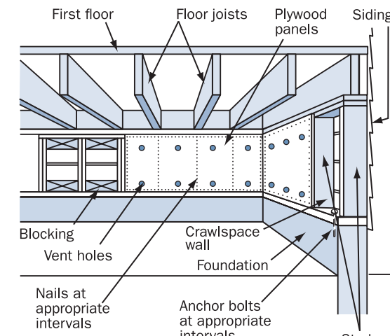
Figure A. Strengthening weak crawlspace walls.
